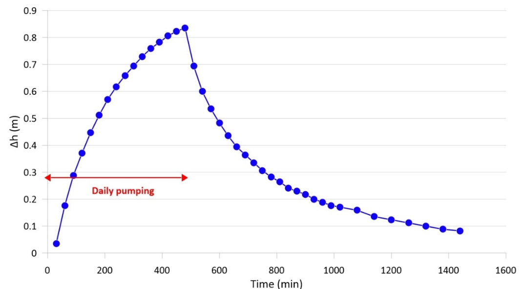
Figure 6. Example of daily drawdown–time curve of Regina Lake level ( \Delta h ) during the spa season.
