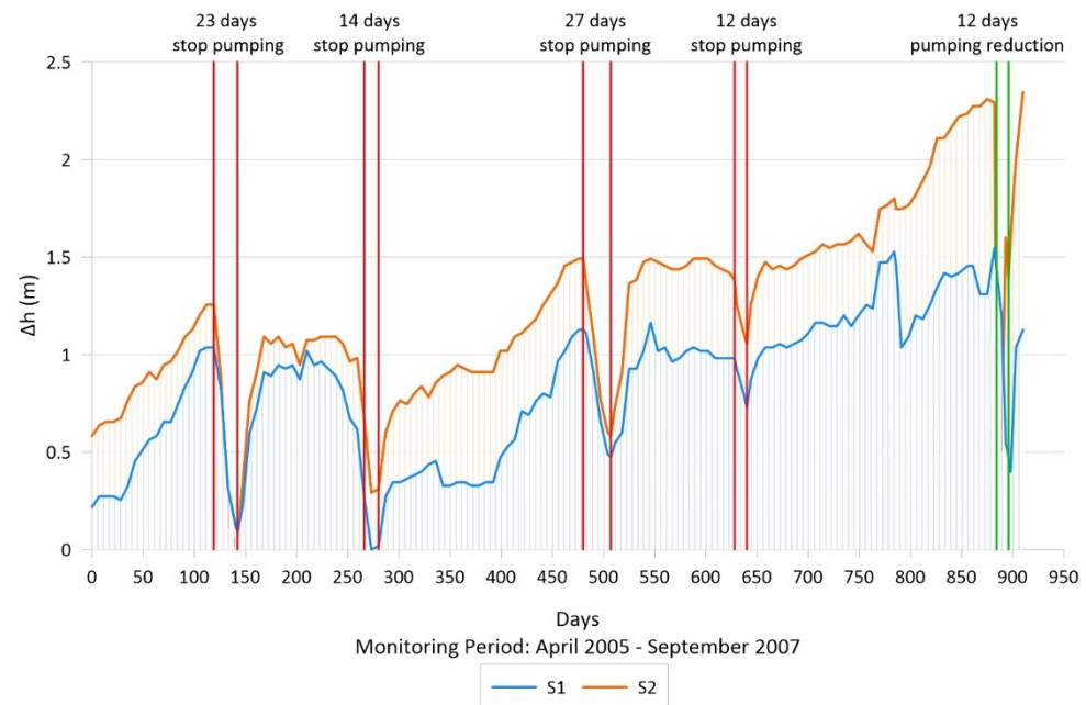
Figure 5. Drawdown fluctuations in two piezometers ( \Delta h ) during the period April 2005–September 2007, showing the groundwater level response to temporary interruption (red lines) of or reduction (green lines) in pumping from the quarry area (from [47]).
