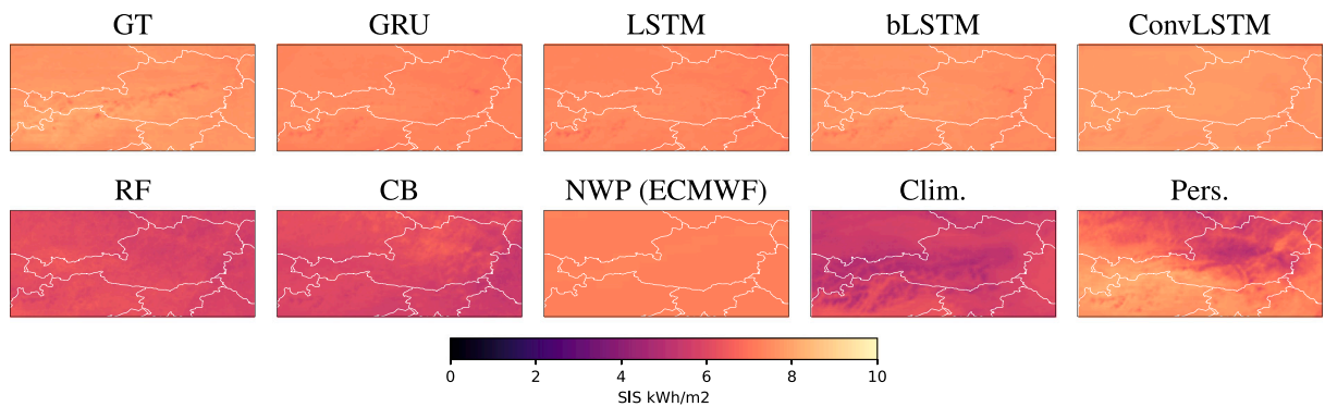
Fig. 9. Daily surface irradiation over Austria at summer time for 2013-08-01 (validation dataset).
