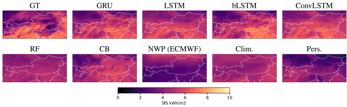
Fig. 6. Daily surface irradiation over Austria at spring time for 2013-05-03 (validation dataset). The satellite ground truth is indicated as GT, for the other acronyms refer to text.
