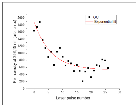
Fig. 4. Stratigraphic LIBS analysis of iron for sample GC.
