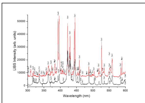
Fig. 3. LIBS spectra of the substrate (black) and of the black crust (red) for sample GP
