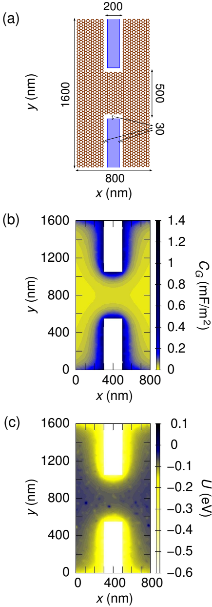
Figure 13. (a) Sketch of the region of the side-gate biased graphene sample for which transport simulations have been performed. The represented hexagonal lattice is not to scale. (b) Map (in the region of the device sketched in panel (a)) of the capacitance per unit area C_G(x, y) between the double side-gate and the point (x, y) of the graphene sample, as a function of the coordinates x and y of the point. (c) Map (in the region of the device sketched in panel (a)) of the graphene potential energy profile U(x, y) obtained for V_G = 90 V.
