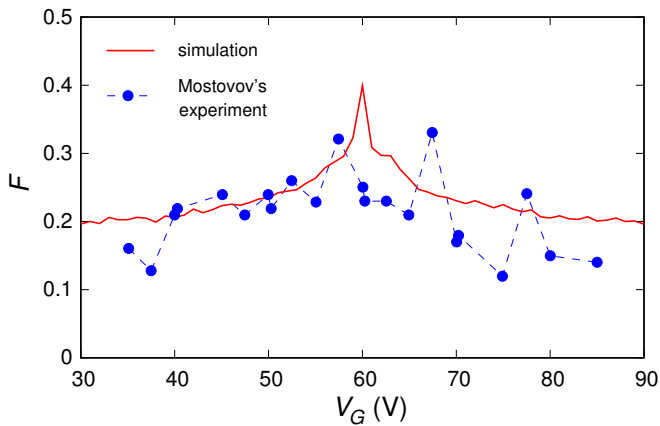
Figure 14. Fano factor F as a function of the gate voltage V_G . Our numerical results are shown with a red solid line, while the experimental results of Mostovov, extracted from Fig. 9.7 of Ref. 19 , are reported with blue dots.
