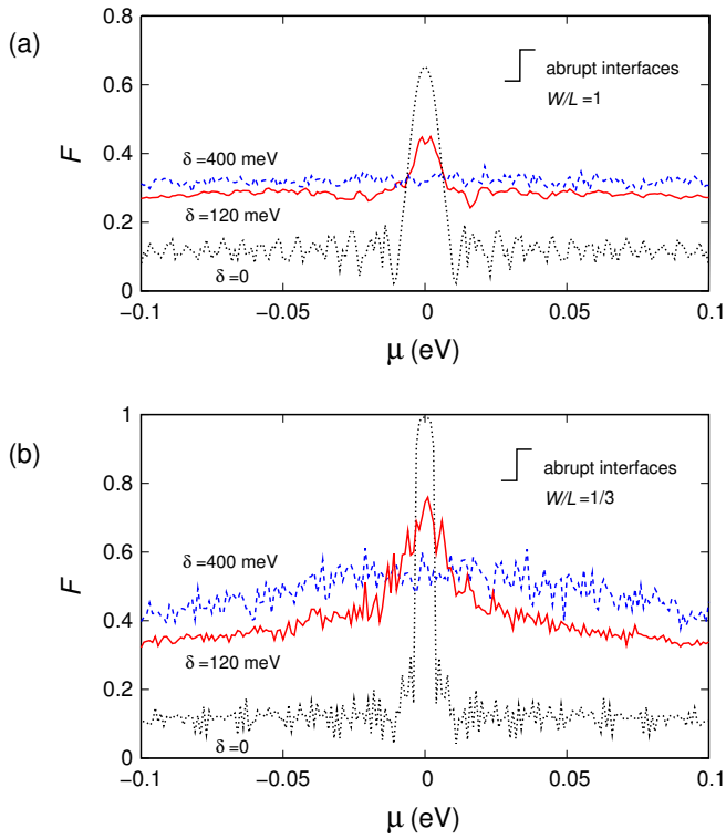
Figure 4. Fano factor as a function of the potential energy \mu in a 200 nm wide armchair ribbon with a length of 200 nm (panel (a)) and 600 nm (panel (b)). The Fermi energy is set to 0 eV and abrupt lead-sample interfaces are assumed. The dotted black curves have been obtained in the absence of disorder, the red solid ones in the presence of a disorder with c_{imp} = 5 \times 10^{11} \text{ cm}^{-2} , HWHM = 5 nm and \delta = 120 \text{ meV} , and the blue dashed ones in the presence of a disorder with c_{imp} = 5 \times 10^{11} \text{ cm}^{-2} , HWHM = 5 nm and \delta = 400 \text{ meV} . The results have been obtained by averaging over 48 different impurity distributions.
