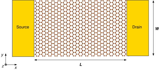
Figure 1. Sketch of a W -wide and L -long armchair graphene ribbon connected to source and drain contacts.
