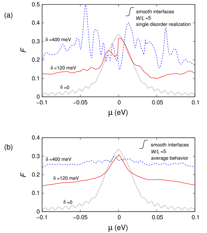
Figure 3. Same as Fig. 2 for smooth lead-sample interfaces.
