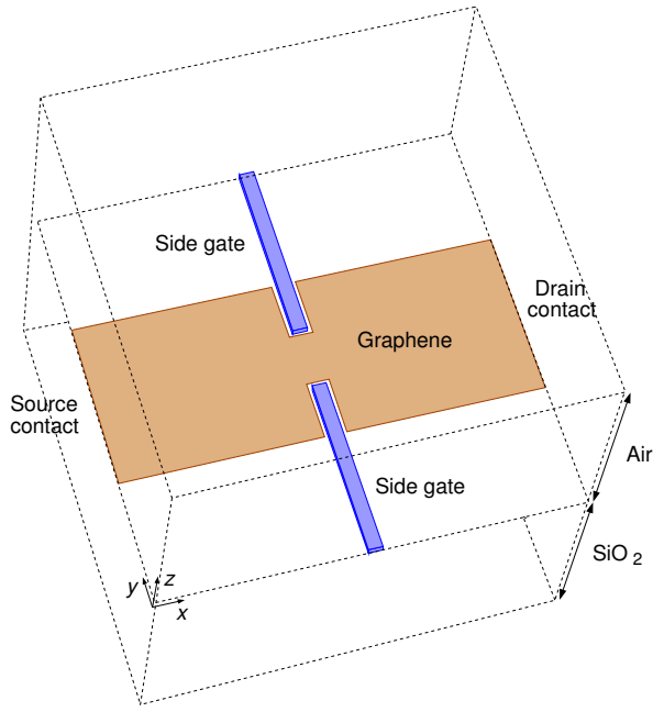
Figure 12. Geometry of the simulated side-gate structure, modeling the device experimentally studied by Mostovov 19 .
