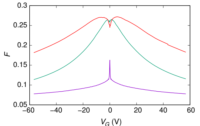
Figure 9. Fano factor, obtained averaging both noise and conductance over a window of 30 meV before taking their ratio, represented as a function of applied back-gate voltage V_G for a 200 nm long and 1000 nm wide graphene flake ( W/L = 5 ) in the absence of disorder (purple line), in the presence of the intermediate disorder (green line), and in the presence of the stronger disorder (red line) specified in Fig. 6.
