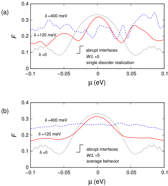
Figure 2. Fano factor as a function of the potential energy \mu in a 40 nm long and 200 nm wide armchair ribbon. The Fermi energy is set to 0 eV and abrupt lead-sample interfaces are assumed. The dotted black curves have been obtained in the absence of disorder, the solid red ones in the presence of a disorder with c_{imp} = 5 \times 10^{11} \text{ cm}^{-2} , HWHM = 5 nm and \delta = 120 \text{ meV} , and the dashed blue ones in the presence of a disorder with c_{imp} = 5 \times 10^{11} \text{ cm}^{-2} , HWHM = 5 nm and \delta = 400 \text{ meV} . Panel (a) reports the results obtained for a single impurity distribution, while the results in panel (b) have been obtained by averaging over 48 different impurity distributions.
