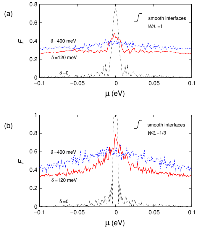
Figure 5. Same as Fig. 4 for smooth lead-sample interfaces.
