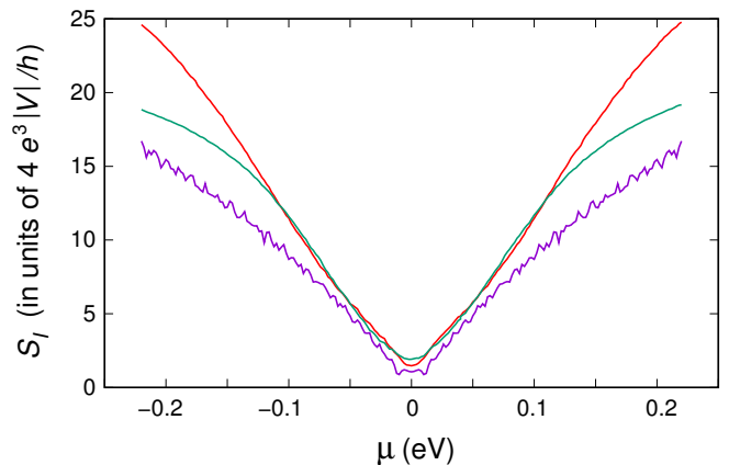
Figure 11. Shot noise power spectral density as a function of the potential energy \mu for a graphene flake 200 nm long and 1000 nm wide ( W/L = 5 ) in the absence of disorder (purple line), in the presence of the intermediate disorder (green line), and in the presence of the stronger disorder (red line) considered in Fig. 6.
