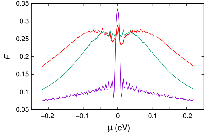
Figure 6. Fano factor as a function of the potential energy \mu for a 200 nm long and 1000 nm wide graphene flake ( W/L = 5 ) in the absence of disorder (purple line), in the presence of an intermediate disorder with c_{imp} = 5 \times 10^{11} \text{ cm}^{-2} , HWHM = 10 nm and \delta = 50 \text{ meV} (green line), and in the presence of a stronger disorder with c_{imp} = 5 \times 10^{11} \text{ cm}^{-2} , HWHM = 5 nm and \delta = 120 \text{ meV} (red line).
