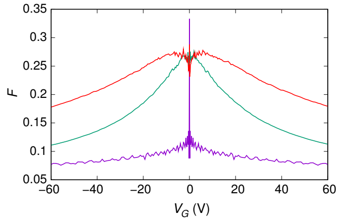
Figure 8. Fano factor as a function of the applied back-gate voltage V_G for a 200 nm long and 1000 nm wide graphene flake ( W/L = 5 ) in the absence of disorder (purple line), in the presence of the intermediate disorder (green line), and in the presence of the stronger disorder (red line) specified in Fig. 6.
