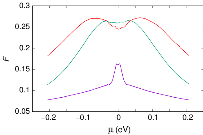
Figure 7. Fano factor, obtained averaging both noise and conductance over a window of 30 meV before taking their ratio, represented as a function of the potential energy \mu for a 200 nm long and 1000 nm wide graphene flake ( W/L = 5 ) in the absence of disorder (purple line), and in the presence of the intermediate disorder (green line), and of the stronger disorder (red line) specified in Fig. 6.
