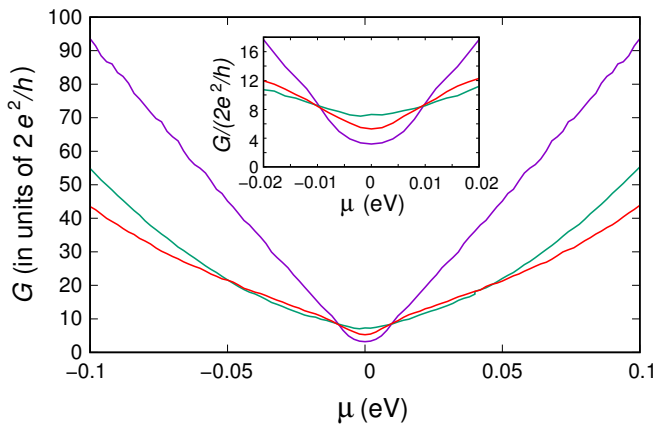
Figure 10. Conductance as a function of the potential energy \mu for a 200 nm long and 1000 nm wide graphene flake ( W/L = 5 ) in the absence of disorder (purple line), in the presence of the intermediate disorder (green line), and in the presence of the stronger disorder (red line) specified in Fig. 6.
