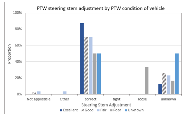
Fig. 14. PTW steering stem adjustment
