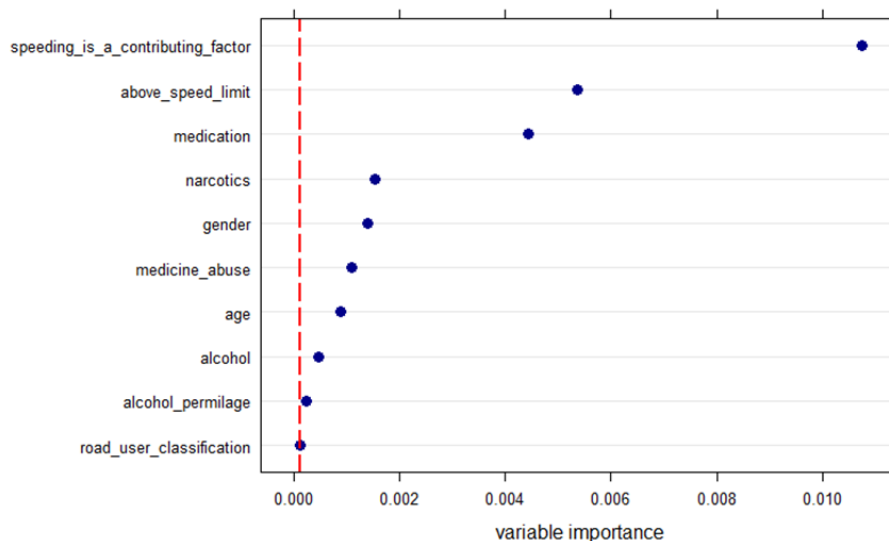
Fig. 20. Variable importance ranking from Random Forest analysis
