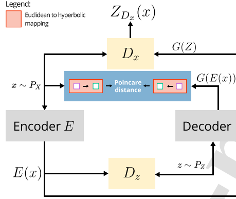
Figure 4: Overall architecture of our proposed model HypAD.
