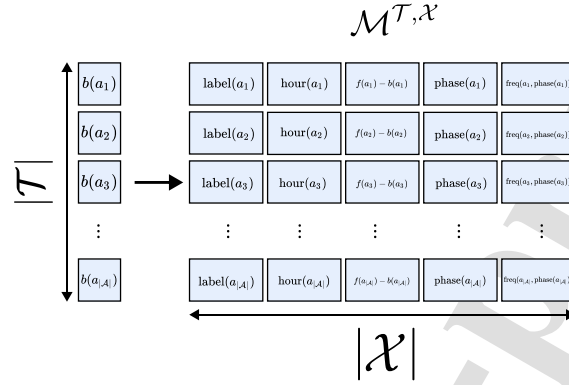
Figure 2: Input modelling of an activity sequence to get a multivariate time series.
