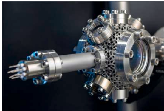
Fig. 24. Additively manufactured vacuum system incorporating cellular design for lightweighting and heat transfer [263].
