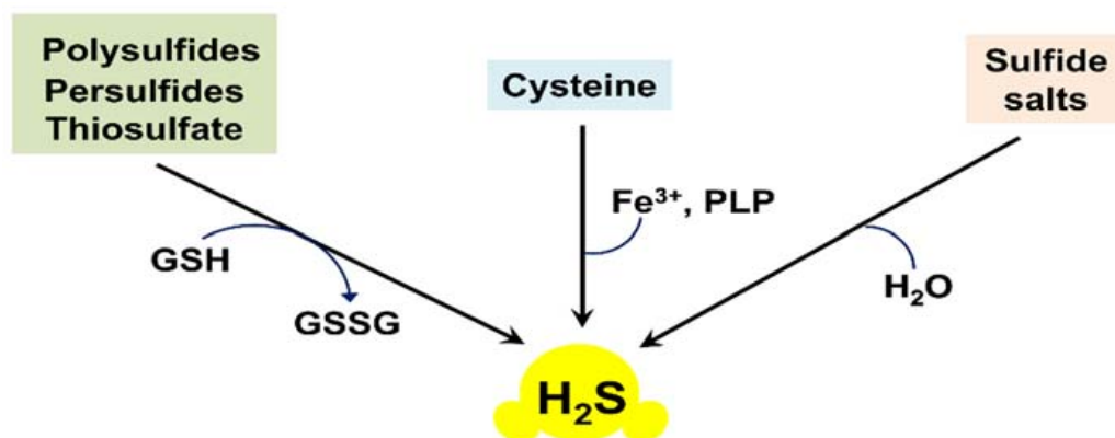
Figure 2. Non-enzymatic endogenous production of H 2 S in mammalian tissues.
