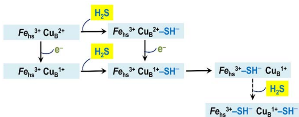
Figure 5. Proposed mechanism of inhibition of mitochondrial cytochrome c oxidase and Escherichia coli cytochrome bo 3 by H 2 S. Shown is the catalytic binuclear center in different redox and ligation states. The center consists of the copper ion Cu B and the high-spin heme ( Fe hs ). The latter is heme a 3 in cytochrome c oxidase and heme o 3 in cytochrome bo 3 . The metal redox groups which are not part of the center are not shown.
