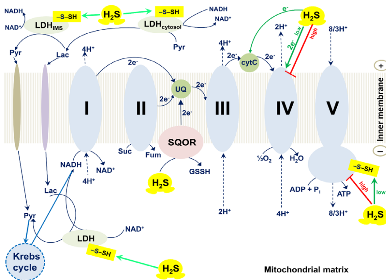
Figure 4. Effects of H 2 S on mammalian mitochondrial electron transport chain, ATP synthase, and lactate dehydrogenase. The mammalian respiratory chain includes four different membrane-bound complexes: I, II, III, and IV. H 2 S at low concentrations stimulates the activity of F 0 F 1 -ATP synthase (also known as complex V) via S-sulphydration of Cys244 or Cys294 of its \alpha subunit [30]. H 2 S increases the activity of lactate dehydrogenase (LDH) via S-sulphydration of its Cys163 that, in turn, stimulates mitochondrial electron transport [31]. H 2 S can also donate electrons to the respiratory chain via sulfide quinone oxidoreductase (SQOR) by directly reducing ubiquinone (UQ) [32]. At high (toxic) concentrations H 2 S inhibits complex IV (cytochrome c oxidase) and F 0 F 1 -ATP synthase that leads to reversible inhibition of mitochondrial electron transport and ATP production [30,33–35]. At low concentrations H 2 S serves as an electron donor for complex IV, either directly [36–38] or indirectly, via reduction of its native substrate cytochrome c [39]. The outer mitochondrial membrane is not shown for simplicity.
