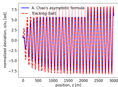
Figure 2: Transverse oscillations of the tail in strong BBU regime: comparison with the asymptotic formula in [3].
