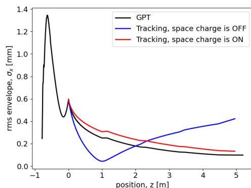
Figure 1: The effect of transverse space charge forces. Injection in the 4 section linac occurs at z = 0 .
