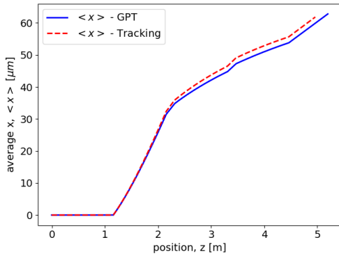
Figure 3: Center of mass transverse displacement induced by a misaligned section ( \Delta x_2 = 50 \mu\text{m} , \delta_2 = 50 \mu\text{rad} ).
