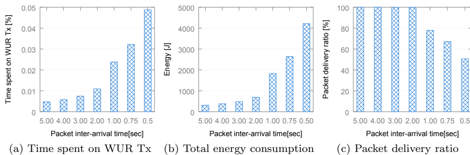
Figure 6: Performance analysis of G-WHARP for varying packet inter-arrival time.
