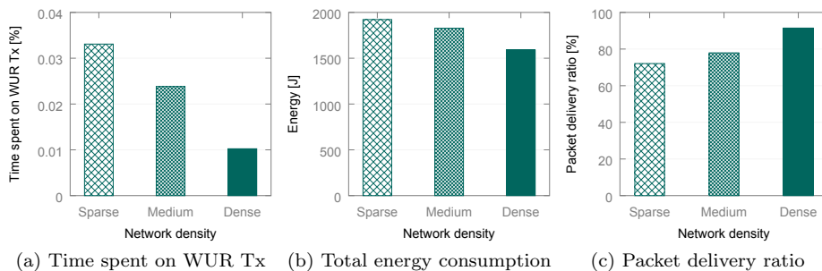
Figure 4: Performance analysis of G-WHARP for varying network density.
