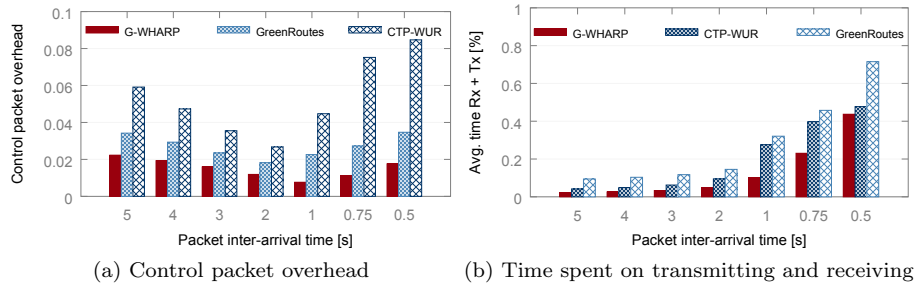
Figure 7: Control packet overhead and time spent with the main radio on.
