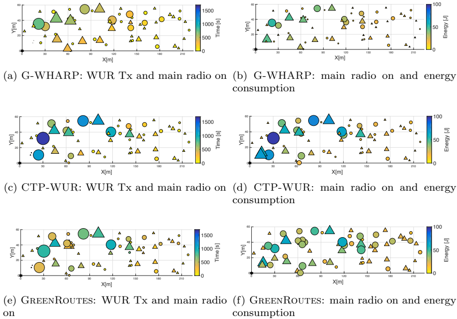
Figure 9: Per node snapshots: G-WHARP vs. CTP-WUR vs. GREENROUTES.
