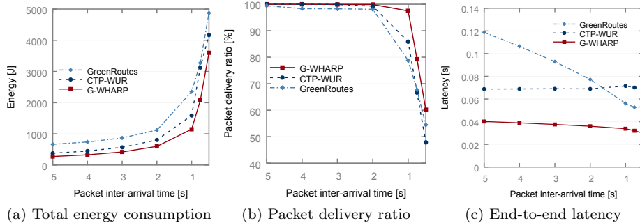
695 Figure 8: Total energy consumption, packet delivery ratio, and end-to-end latency.
