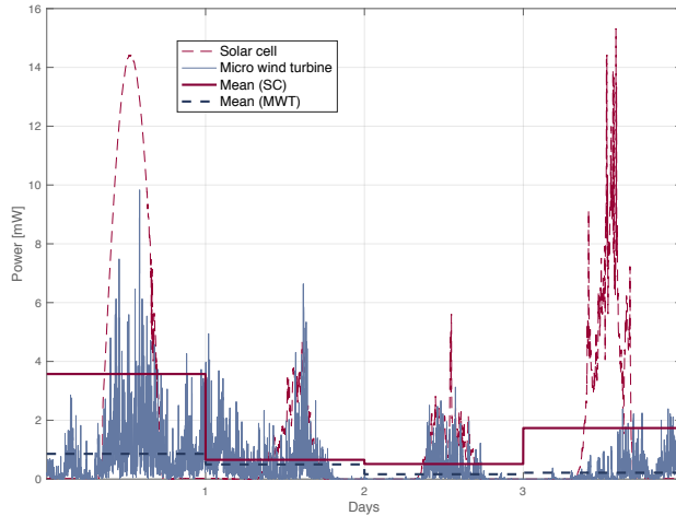
Figure 2: Sample of harvested power: Solar vs. wind.
