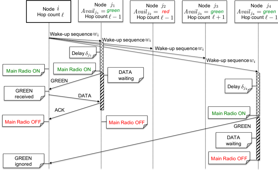
Figure 1: G-WHARP forwarding: An example.
