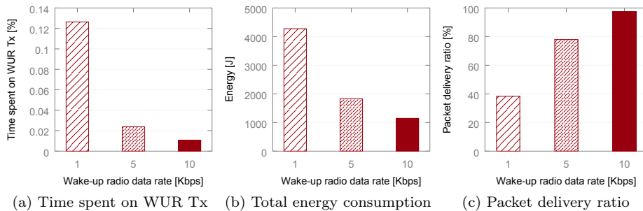
Figure 5: Performance analysis of G-WHARP for varying wake-up radio data rate.
