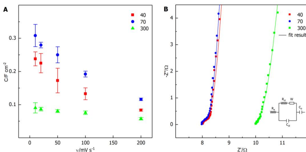
Figure 4: A) Capacitance values obtained from cyclic voltammetry experiments carried out at different scan rates. B) Nyquist plot recorded for the different electrodes.
