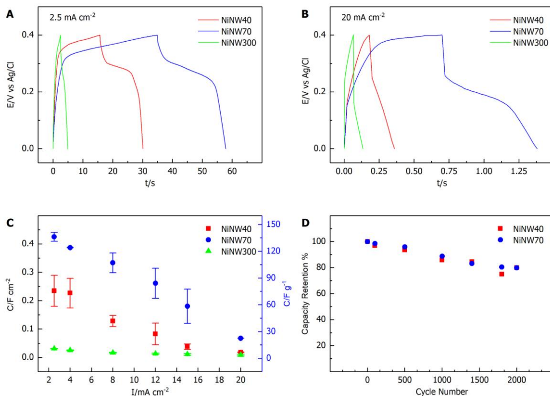
Figure 5: Charge-discharge curves at 2.5 \text{ mA cm}^{-2} (A) and 20 \text{ mA cm}^{-2} (B). C) Obtained capacitance from galvanostatic charge-discharge at different current densities. D) Capacitance retention of the NiNW40 and NiNW70 electrodes at 20 \text{ mA cm}^{-2}
