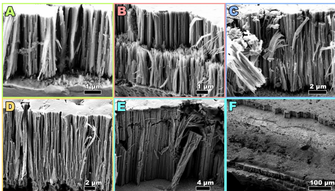
Figure 6: SEM cross-sectional images of the NiNW obtained by electrodeposition using alumina template produced with different anodization times.
