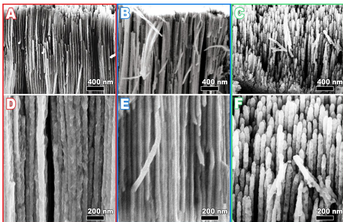
Figure 1: SEM cross-sectional images of the Ni NWS electrodes treated at 40 °C (A, D), 70°C (B, E) and 300°C (C, F).
