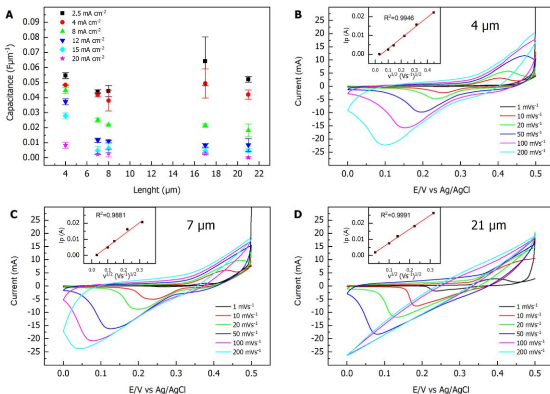
Figure 8. A) Capacitance values normalized per nanowires length. Cyclic voltammetry performed at different scan rate of electrode with nanowires length of 4 (B), 7 (C) and 21 (D) \mu m . Inset graph report the linear trend between cathodic peak current and the square root of scan rates
