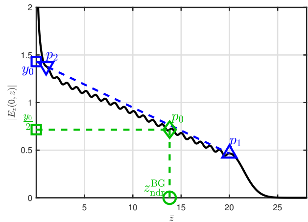
FIG. 10. Schematic representation of a typical field-amplitude decay |E_z(0, z)| along the z -axis for a BGB. The numerical procedure employed for the calculation of z_{\text{ndr}}^{\text{BG}} is schematically reported in the figure and explained in detail in the text.
