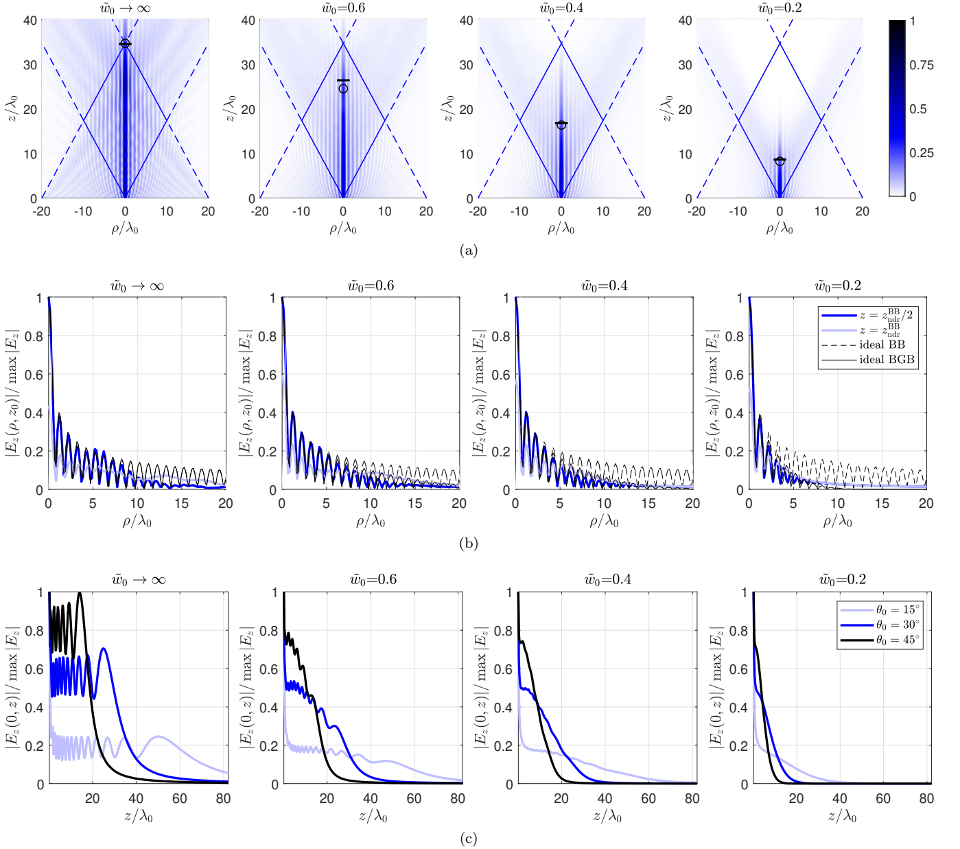
FIG. 3. (a) Color maps of the absolute value of the E_z component of the electric field over the xz -plane in the range |\rho| < \rho_{\text{ap}} = 20\lambda_0 and 0 < z < 40\lambda_0 . From left to right, \tilde{w}_0 decreases from a very large value (close to the asymptotic condition for having a BB, i.e., \tilde{w}_0 \rightarrow \infty ) up to \tilde{w}_0 = 0.2 (close to the asymptotic condition for having a GB, i.e., \tilde{w}_0 \rightarrow 0 ). The black bars and circles represent the numerical calculations and analytical estimations through (8) of z_{\text{ndr}}^{\text{BB}} , respectively. (b) Radial 1-D electric field profiles at z_0 = z_{\text{ndr}}^{\text{BB}}/2 (blue solid lines) and z_0 = z_{\text{ndr}}^{\text{BB}} (light blue solid lines) for different values of \tilde{w}_0 from left to right (the same as in (a)). The electric field profiles are normalized to their respective maxima for each different value of \tilde{w}_0 , and compared with the theoretical profiles of an ideal BB (black dashed line) and an ideal BGB (black solid line). (c) On-axis 1-D electric field profiles for different \tilde{w}_0 from left to right (the same as in (a)), and different axicon angles \theta_0 = 15^\circ , \theta_0 = 30^\circ , \theta_0 = 45^\circ , in light blue, blue, and black solid lines, respectively.
