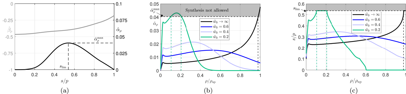
FIG. 7. (a) Normalized phase and attenuation constants of the radiative space harmonic of the fundamental TM leaky mode supported at f = 18 GHz by a linearized BE structure as in Fig. 6 with radial period p = 10 mm, substrate thickness h = 3.14 mm, and substrate relative permittivity \varepsilon_r = 2.2 , as a function of the ratio between the strip width s and p . (b) Radial profiles of the normalized attenuation function required for synthesizing a BGB aperture field as in (13), for different values of the normalized beam waist \tilde{w}_0 . (c) Radial profiles of the ratio s/p corresponding to the cases shown in (b).
