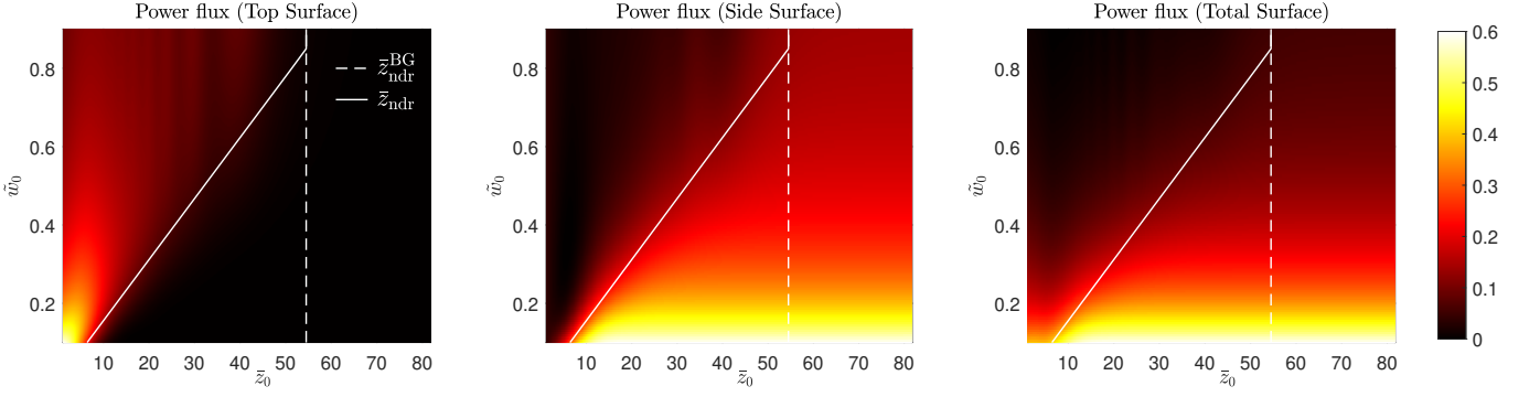
FIG. 5. From left to right, the power flux over the top surface \int_{\Sigma_T} d\sigma S_z , the power flux over the side surface \int_{\Sigma_S} d\sigma S_\rho , and the power flux over the whole surface ( \int_{\Sigma_T} d\sigma S_z + \int_{\Sigma_S} d\sigma S_\rho ) (each normalized to the power through the entire radiating aperture \int_{\Sigma_A} d\sigma S_z ) are shown as a function of \tilde{z}_0 = z_0/\lambda_0 and \tilde{w}_0 . The white solid and dashed lines represent the limits set by \tilde{z}_{\text{ndr}}^{\text{BG}} and \tilde{z}_{\text{ndr}} , respectively.
