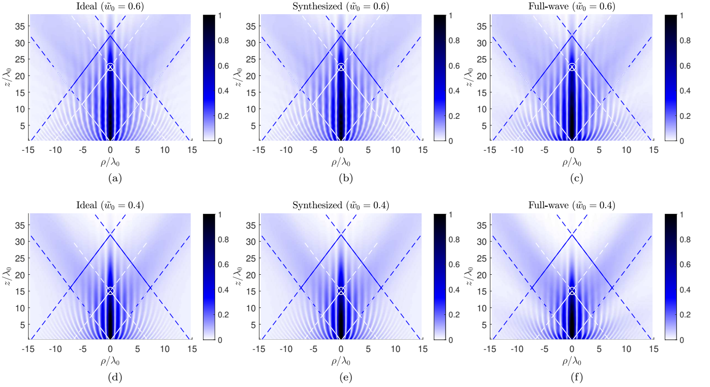
FIG. 8. Colormaps showing the absolute value of E_z in an arbitrary azimuthal \rho z plane, for BGBs having two different values of the normalized waist: \tilde{w}_0 = 0.4 and 0.6 . (a) and (d): fields radiated by the ideal aperture distribution (13); (b) and (e): fields radiated by the aperture distribution synthesized through the radial tapering of the attenuation constant via (12); (c) and (f): full-wave results obtained with CST for the actual BE structure designed as described in Sec. IV-A. The blue dashed lines represent the shadow boundaries expected for a BB (i.e., \tilde{w}_0 \rightarrow \infty ), whereas the white dashed lines represent the shadow boundaries expected for a BGB as predicted by (8). White circles mark the numerical evaluations of z_{\text{ndr}}^{\text{BGB}} (note the close agreement with the intersection point of the shadow boundaries).
