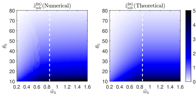
FIG. 2. The nondiffractive range normalized to the aperture radius z_{\text{ndr}}^{\text{BG}} , as a function of \theta_0 and \tilde{w}_0 , is evaluated numerically (on the left) and through (8) (on the right). A vertical dashed white line highlights the limiting value \tilde{w}_0 = \tilde{w}_{0,\text{lim}} .
