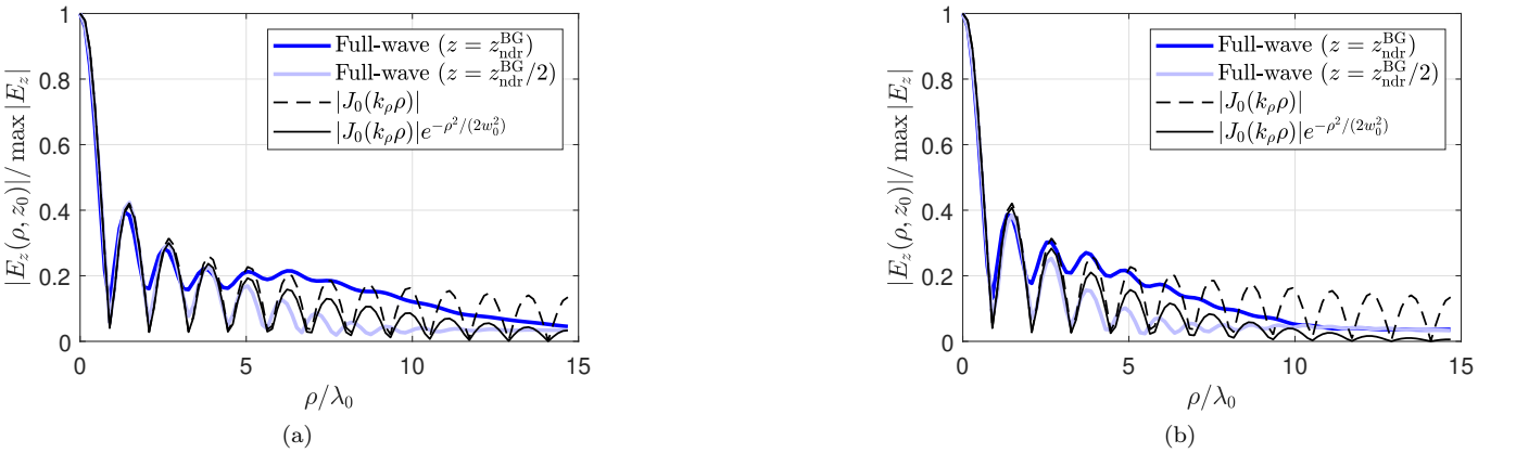
FIG. 9. Transverse radial profiles of |E_z| evaluated at z = z_{\text{ndr}}^{\text{BGB}} and z = z_{\text{ndr}}^{\text{BGB}}/2 for (a) \tilde{w}_0 = 0.6 and (b) \tilde{w}_0 = 0.4 : comparison between full-wave results obtained by simulating in CST an actual BE structure and ideal Bessel and Bessel-Gauss profiles.
