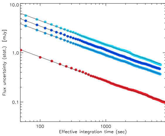
Fig. 17. Comparison of NEFD estimates using two methods on observations of HLS J0918+5142. Left panel: evolution of the 1\sigma flux density uncertainties as a function of the effective integration time t_{\text{eff}} , as defined in Eq. (27), for A1 (cyan), A3 (dark blue), the combination of A1 and A3 (medium blue), and A2 (red). The solid black lines are the best-fit models using \sigma(t_{\text{eff}}) = \text{NEFD} / \sqrt{t_{\text{eff}}} . Right panel: NEFD as a function of the measured line-of-sight atmospheric opacity using the same colour code as in the left panel. The solid black lines are the theoretical fits \text{NEFD}_{\tau_v, x} = \text{NEFD} e^{\tau_v, x} and give the NEFD when extrapolated to \tau_v / \sin(\text{el}) = 0 .
