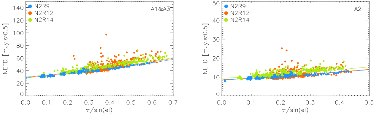
Fig. 18. Comparison of NEFD estimates for three observation campaigns. The measured NEFD using the scatter method is plotted as a function of the line-of-sight atmospheric opacity ( \tau_{\nu,x} ) for the 1 mm ( left ) and 2 mm ( right ) channels. Data points are NEFD estimates in \text{mJy s}^{1/2} for N2R9 (blue), N2R12 (orange) and N2R14 (chartreuse). We also show the expected NEFD evolution with the line-of-sight atmospheric opacity in the plots as solid curves using the median zenith atmospheric opacity derived from all the scans acquired during a campaign.
