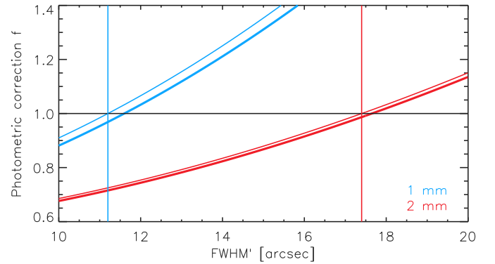
Fig. C.1. Magnitude of the photometric correction f(\sigma) of the beam-variation effect as a function of the actual FWHM, at 1 mm (blue) and 2 mm (red). Thick lines correspond to a choice of \sigma_* derived on a very bright source like Uranus. Thin lines are for sources of 1 Jy at 1 and 2 mm.
