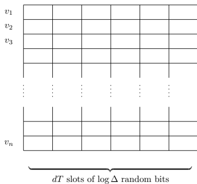
Figure 1: Uncompressed representation \mathcal{M} of R
