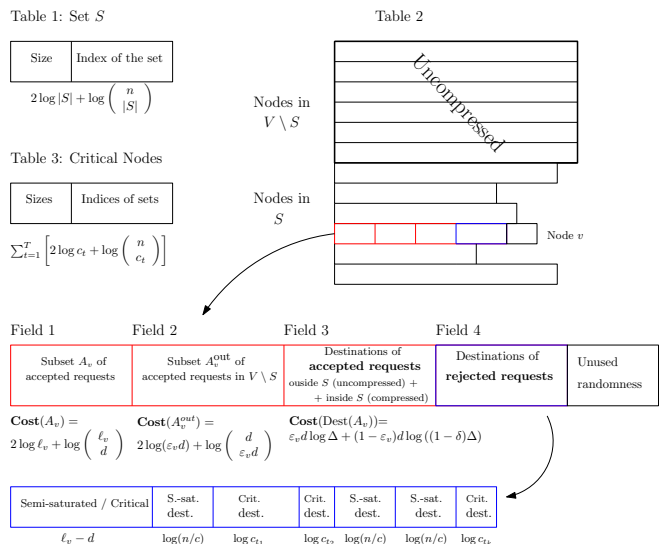
Figure 2: Compressed representation \mathcal{C} of R
