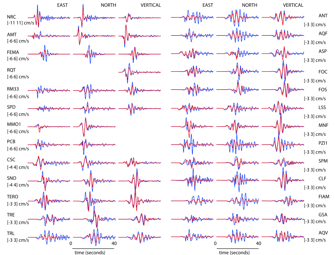
Figure 3. Fit to the data: synthetic ground velocity filtered between 0.02 and 0.5 Hz (red lines) and recorded strong motions (blue lines). Numbers in brackets represent the amplitude range in cm/s for each station.
