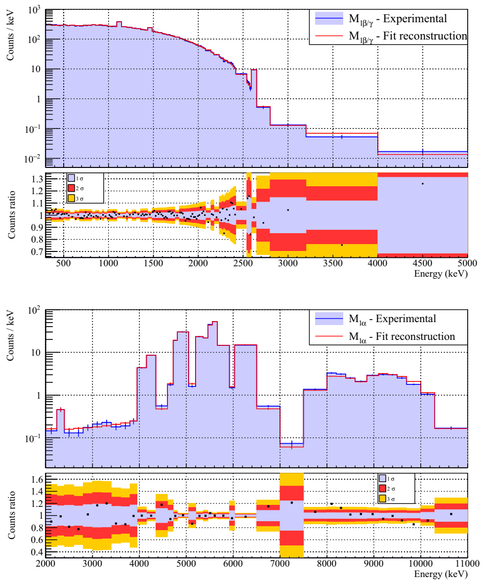
Fig. 5 Top: comparison between experimental \mathcal{M}_{1\beta/\gamma} spectrum and fit reconstruction. The lower panel shows the bin by bin ratios between counts in the experimental spectrum over counts in the reconstructed one; the corresponding uncertainties at 1, 2, 3 \sigma are shown as colored bands centered at 1. Bottom: same as top for \mathcal{M}_{1\alpha} spectrum
