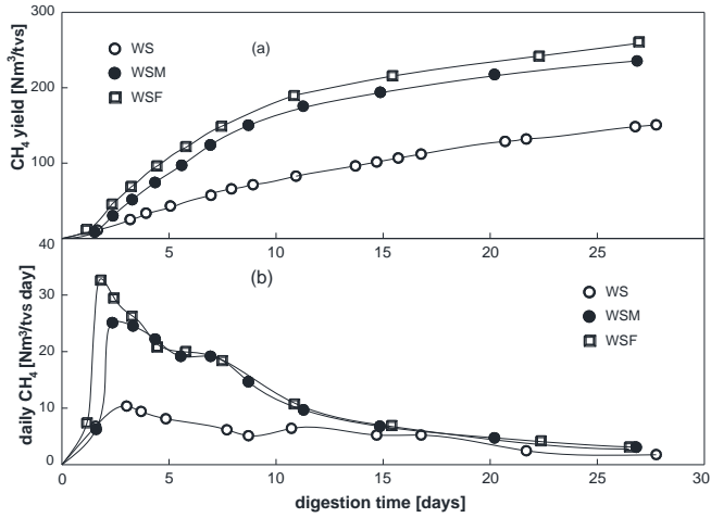
Figure 1. Cumulative (a) and daily (b) methane yield
