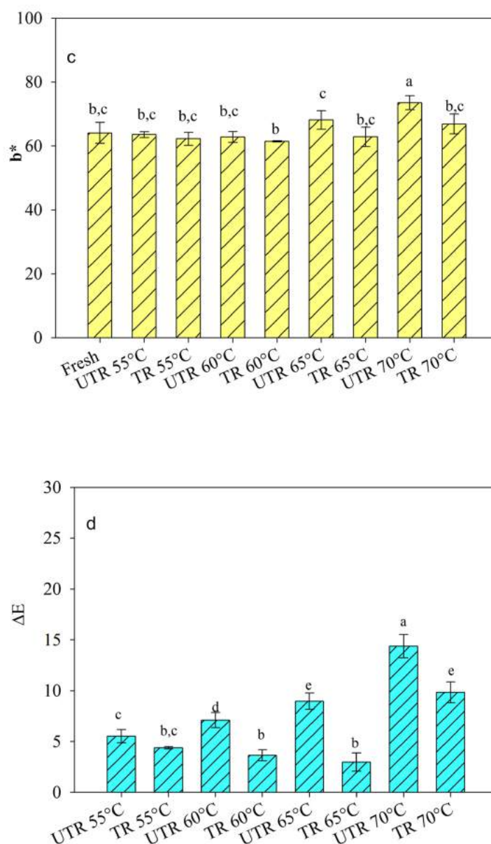
Figure 3. Colour parameters L^* (a), a^* (b), b^* (c) and \Delta E (d) for fresh, untreated (UTR) and pretreated (TR) dried samples at 55, 60, 65 and 70°C.
