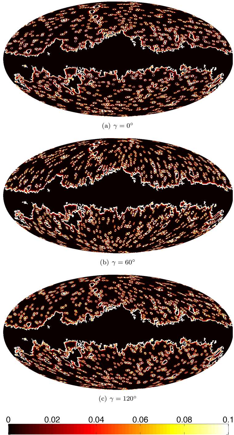
Figure 7: Localisation statistic \Delta^{(j)}(\rho) , plotted using a Mollweide projection for each orientation \gamma , computed from Monte Carlo simulations ( L = 256 , \lambda = 2 , N = 3 , j = 2 ).
