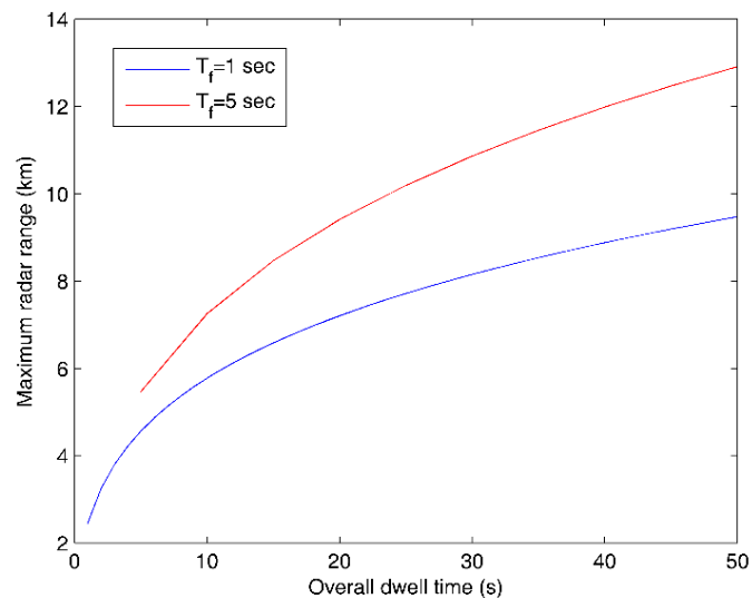
Figure 3.3 - Maximum radar range as a function of overall integration time.
