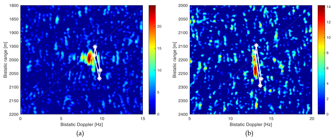
Figure 6.7 - Calculated corner point superimposed on ship RD images obtained for (a) satellite 1 and (b) satellite 2 in case of target radial motion
