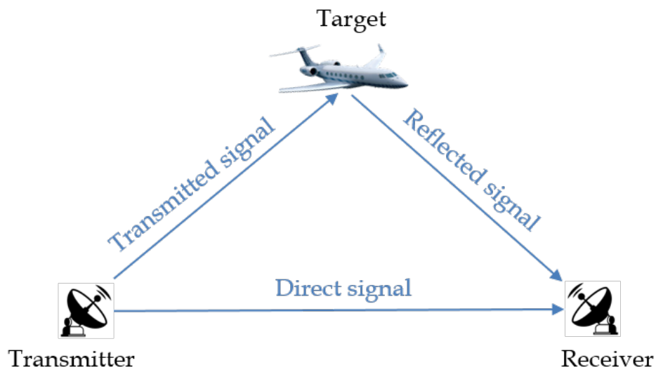
Figure 2.2 - Bistatic radar
