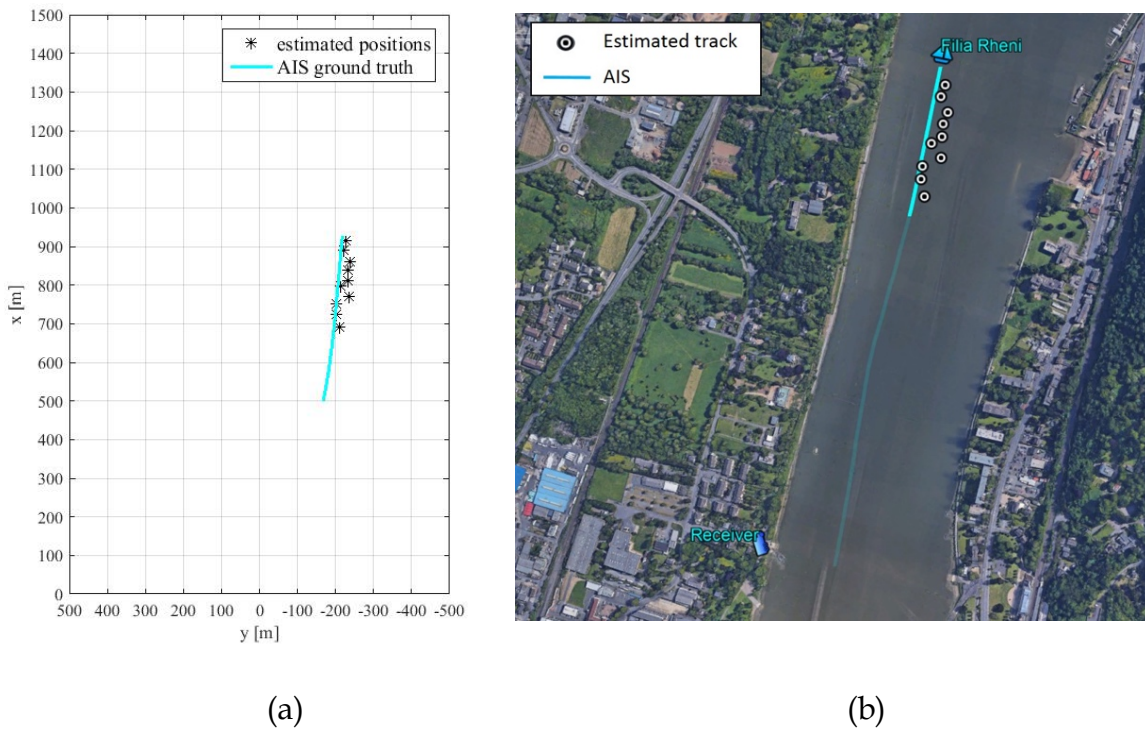
Figure 5.12 - 'Filia Rheni' track. (a) Cartesian plane. (b) Geographical plane.
