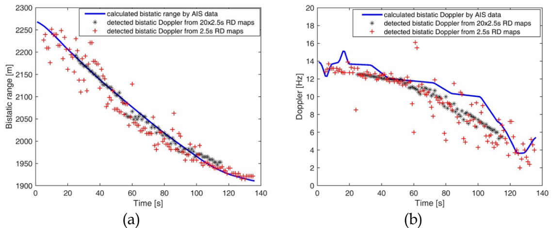
Figure 4.17 - (a) Comparison of bistatic ranges for satellite 2. (b) Comparison of bistatic Doppler for satellite 2
