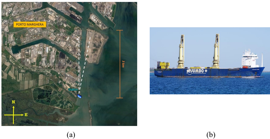
Figure 5.13 - Port operations experimental trials. (a) Acquisition geometry. (b) 'Fairpartner' optical photograph [72].
