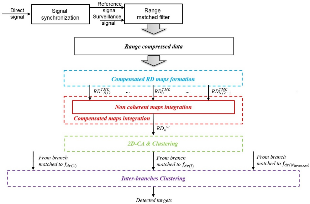
Figure 4.1 - Overall processing chain.
