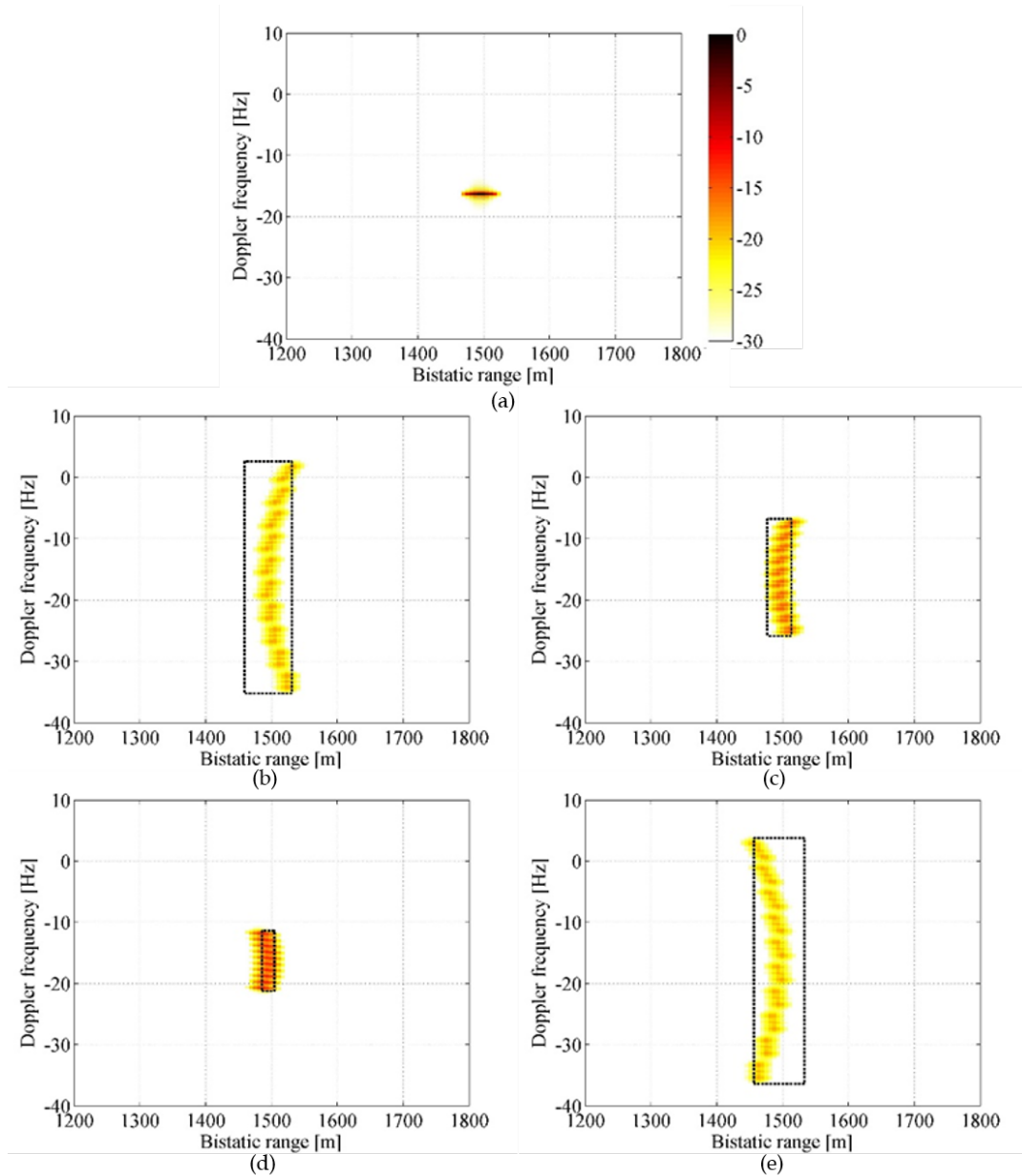
Figure 4.7 - Basic plane maps for different values of the tested Doppler rate. a) f_{dr} = f_{dr_{TG}} = -0.0395 Hz/s; b) f_{dr} = -1.3000 Hz/s; c) f_{dr} = -0.6778 Hz/s; d) f_{dr} = 0.2889 Hz/s; e) f_{dr} = 1.3000 Hz/s.
