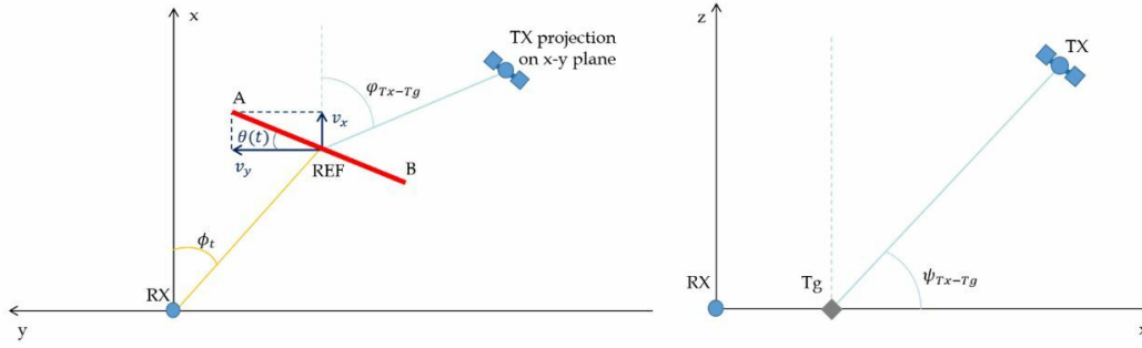
Figure 6.2 - Local reference system.
