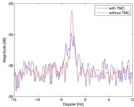
Figure 4.15 - Doppler cross-sections of the sea clutter background.
