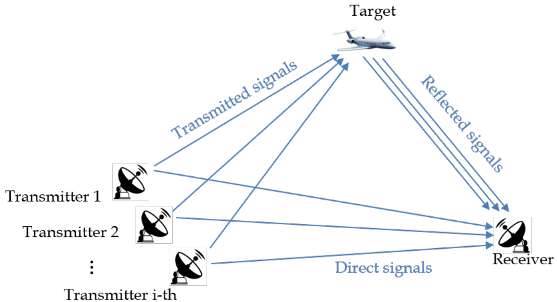
Figure 2.4 – Passive multistatic radar
