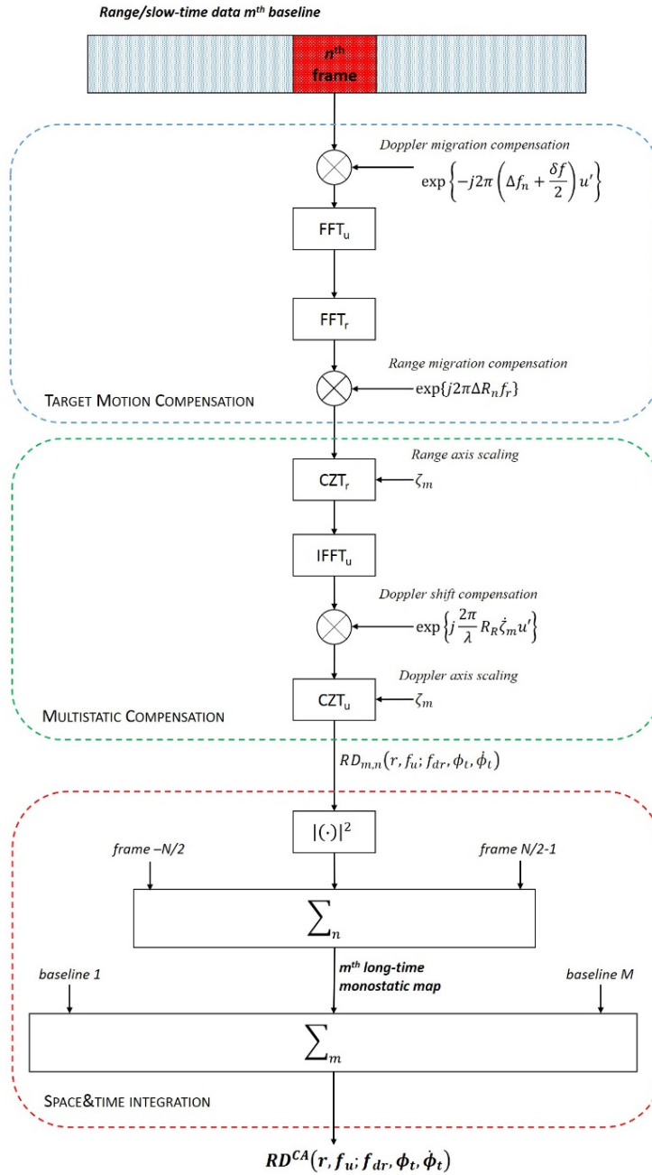
Figure 5.1 - Processing chain
