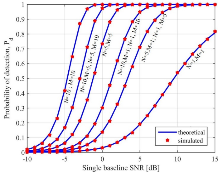
Figure 5.2 - Multi-frame and multi-baseline probability of detection.
