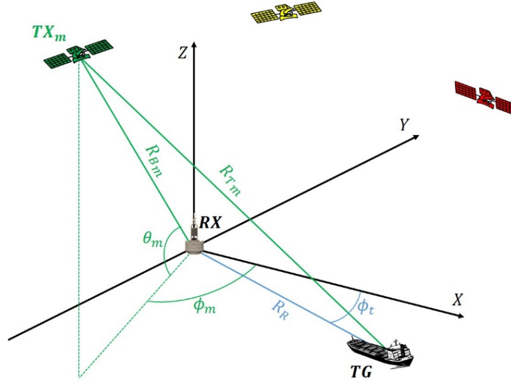
Figure 3.2 - System geometry
