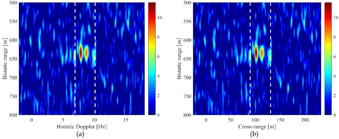
Figure 6.13 - (a) RD image, (b) image after cross-range scaling
