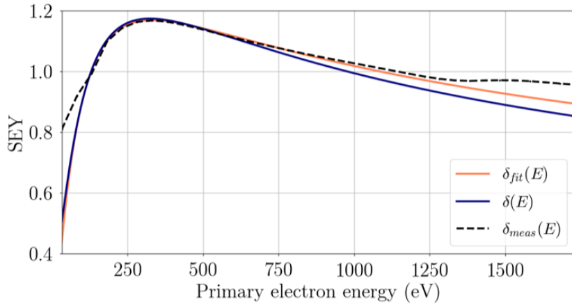
Figure 6.18: Analytic curve for \delta_{max} = 1.16 and LHC chamber parameters (blue), measured curve of the 87 nm film with \delta_{max} = 1.16 and fit curve obtained by modified free parameters.
