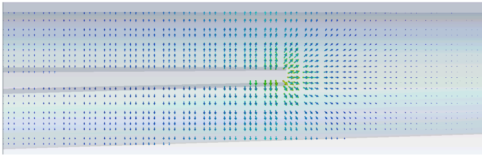
Figure 8.10: Electric field line distribution for the trapped mode in Model 1.
