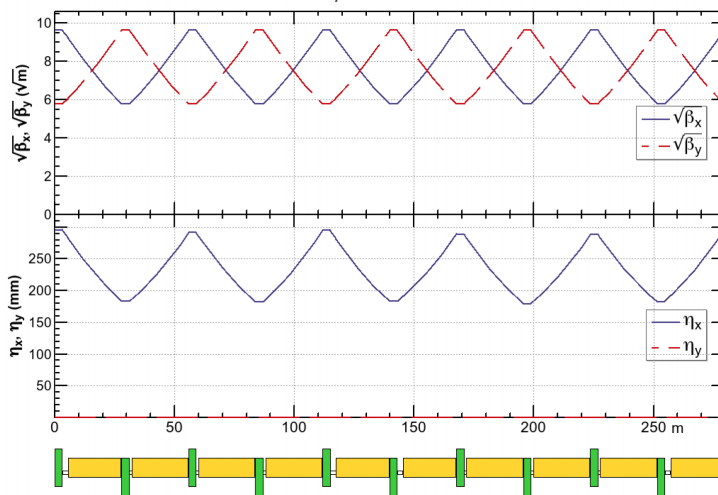
Figure 4.12: Beta functions and dispersion functions along the cells of the FCC-ee arc FODO lattice.
