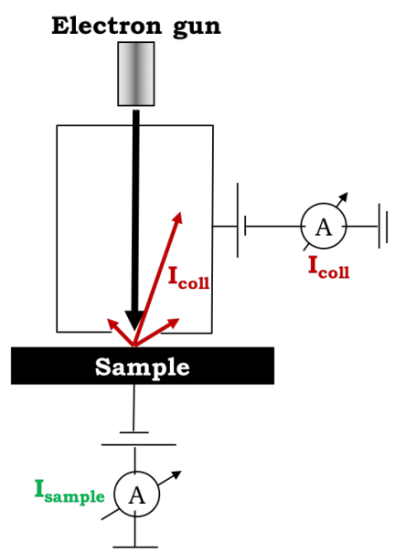
Figure 6.13: Experimental setup for SEY measurements.
