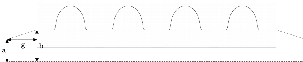
Figure 7.3: Sketch, not in scale, of a group of 4 cells with tapers.
