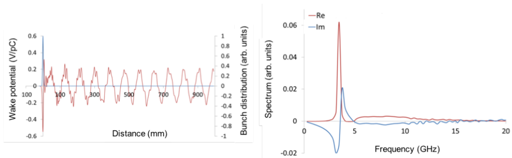
Figure 8.13: Wake potential of a 2.5 mm bunch and spectrum of the excited field in the IR model 3.
