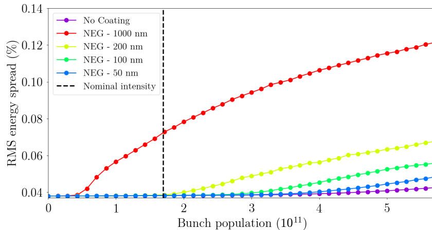
Figure 5.8: RMS energy spread as a function of the bunch population given by numerical simulations considering only the RW impedance in the case of no coating, with a copper pipe of 35 mm radius, and with NEG films at different thicknesses. The dashed black line correspond to the nominal bunch population.
