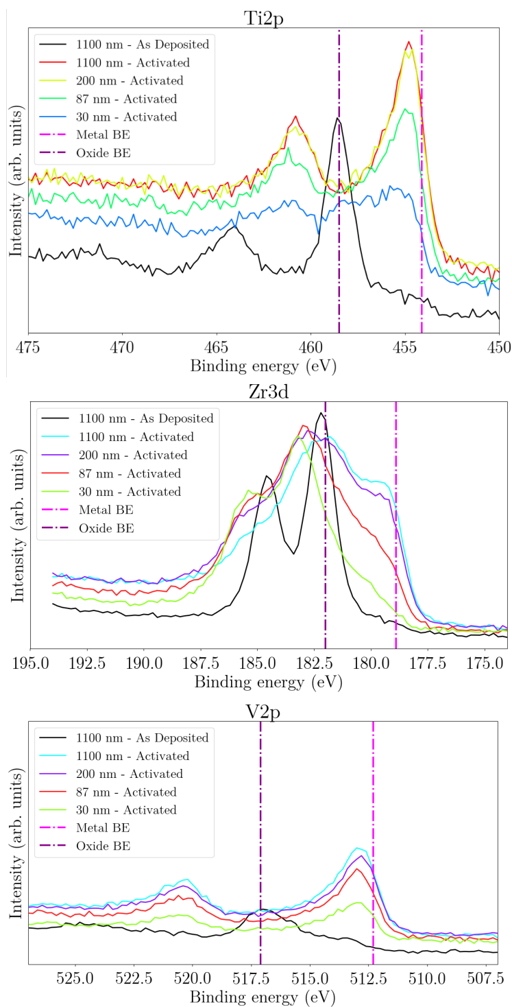
Figure 6.11: Ti2p (top), Zr3d (centre) and V2p (bottom) photopeaks obtained by XPS analysis for all the thicknesses under study. 2p and 3d refer to subshells of electronic configuration.
