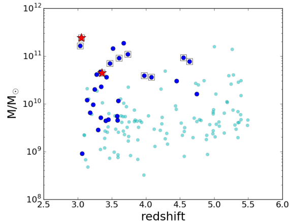
Figure 3. Redshift vs. mass distribution of the red and dead selections. Cyan points refer to objects having z < 5.5 and a passive best-fitting solution (both in the fit including emission lines and in the one without them), but excluded from the reference sample because of the existence of different, non-passive solutions with probability larger than 5%; blue dots: reference sample (30 candidates surviving the probabilistic selection; the void squares mark the 10 sources selected also using the library including nebular lines emission); red stars: the two candidates surviving the free- z fitting. See text for more details.
