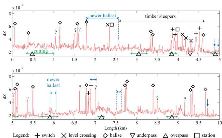
Figure 11. GPR parameter dZ , in frequency domain, regarding data from September 2017 and the identification of track events.
