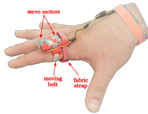
(a) hRing finger device.
