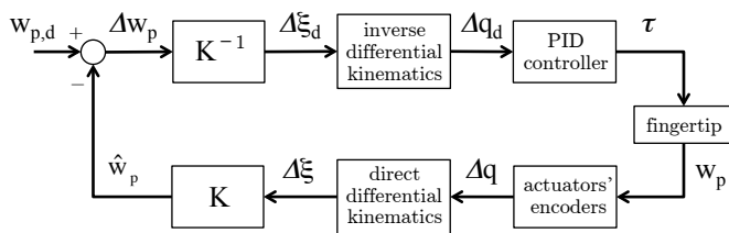
(c) 3-RRS fingertip device control scheme.
